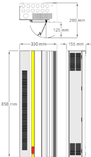
SCA1210 RCBO & RCBOX versions - Consult iLight
