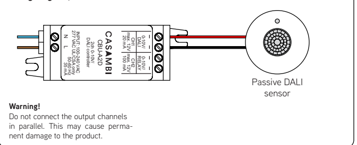
Wiring diagram, DALI sensor
