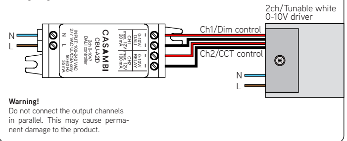
Wiring diagram, 2 channel LED driver
