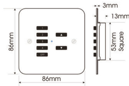
Flush mounting into a 25mm deep standard UK backbox
