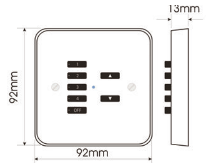
Surface mounting
